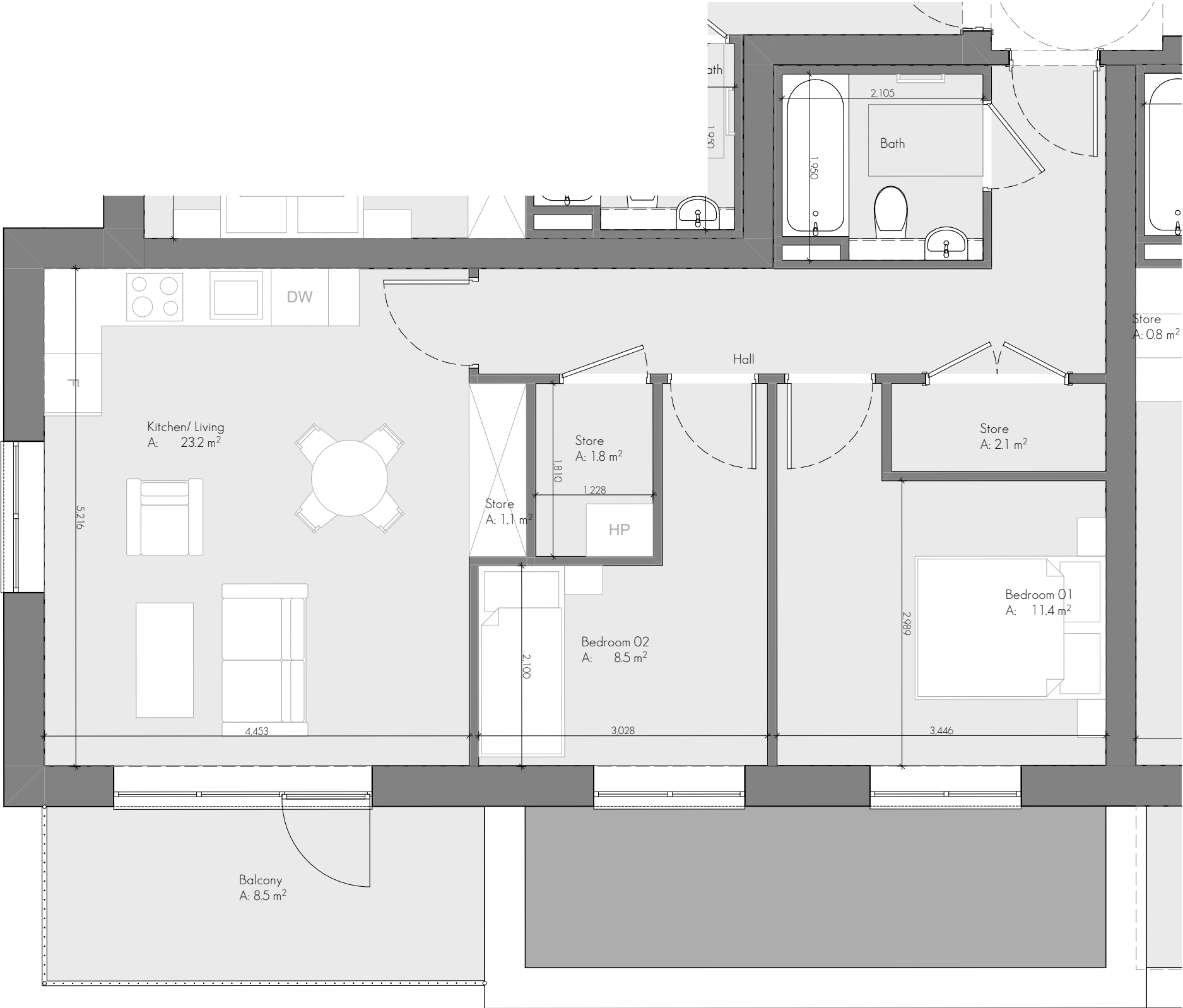
Apartment Type 2F 1:50
