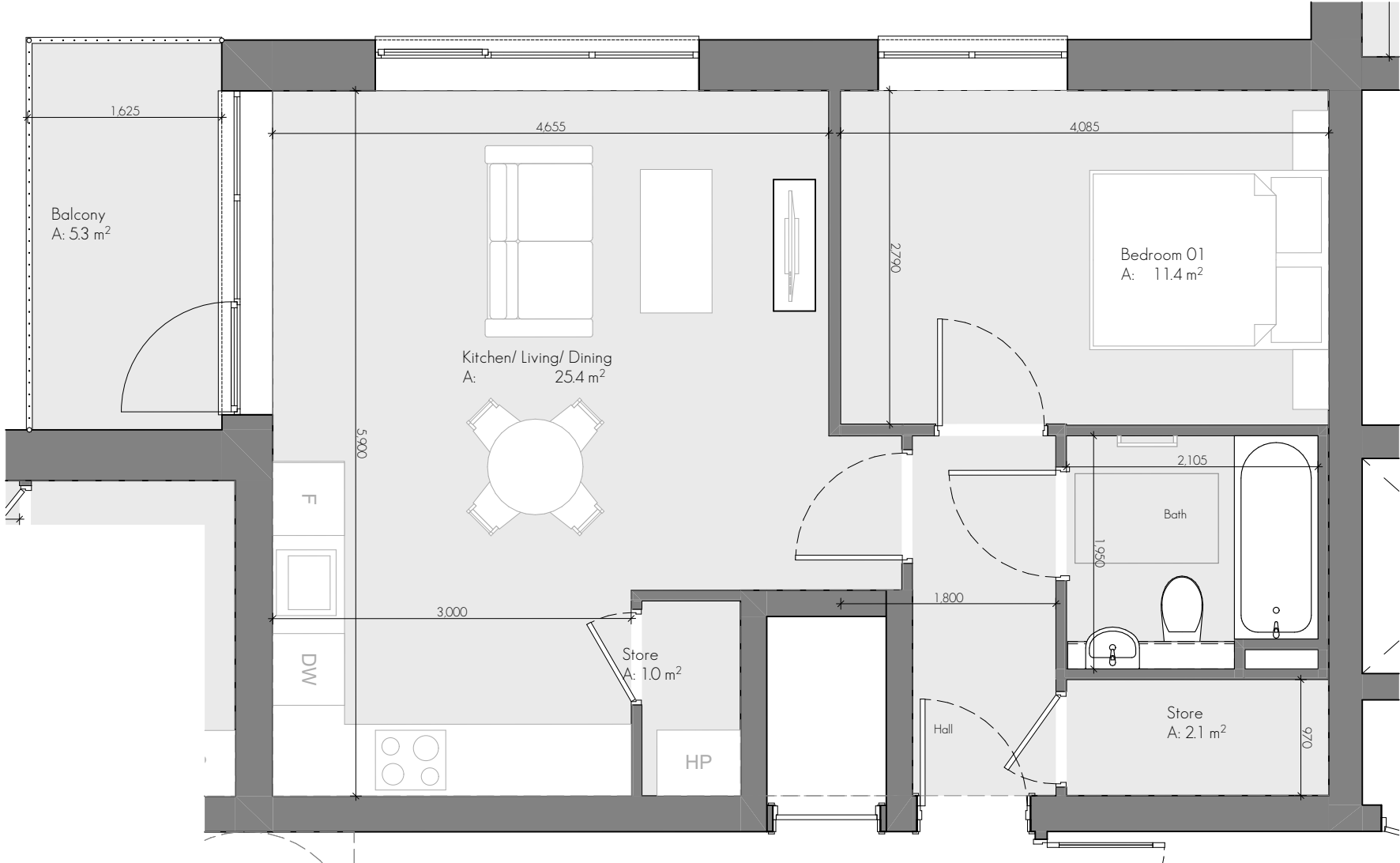
Apartment Type 1C 1:50
