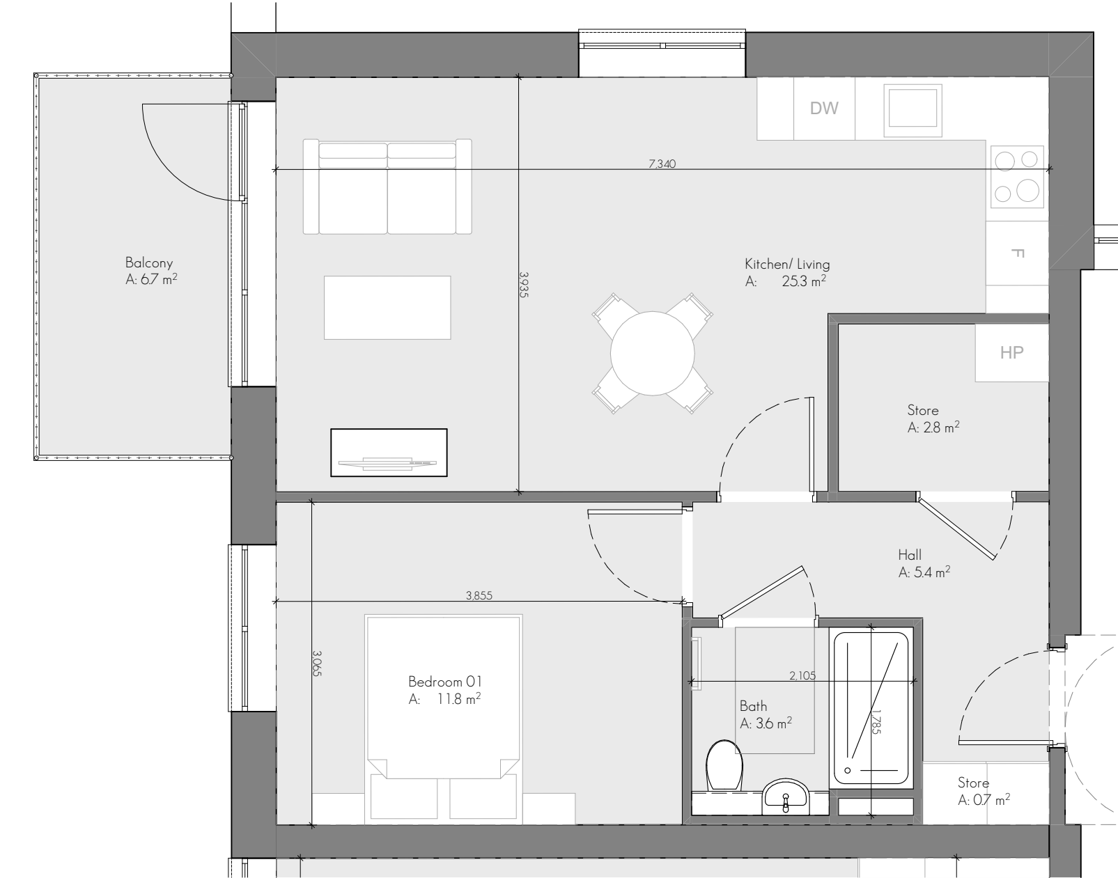
Apartment Type 1A 1:50
