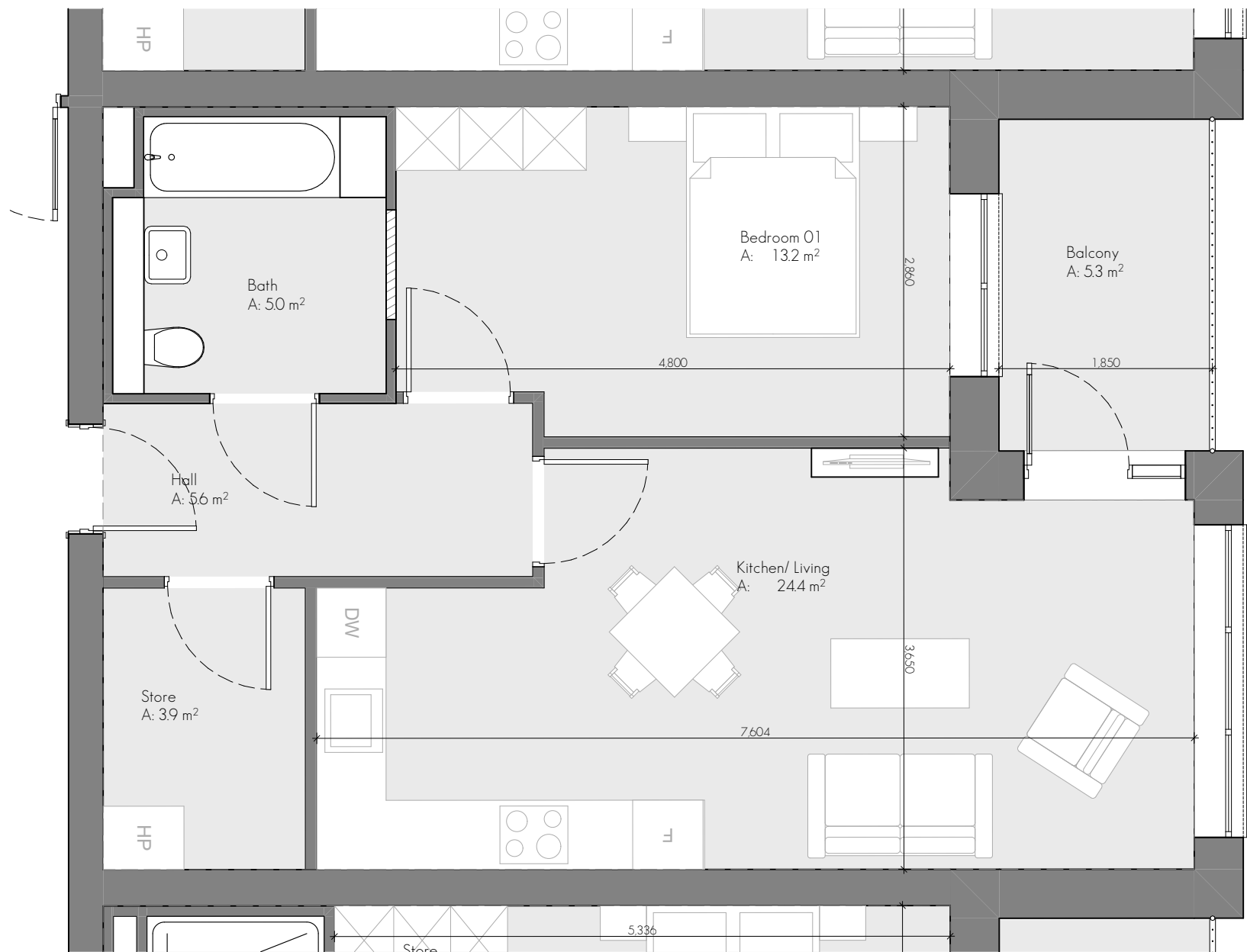
Apartment Type 1B 1:50
