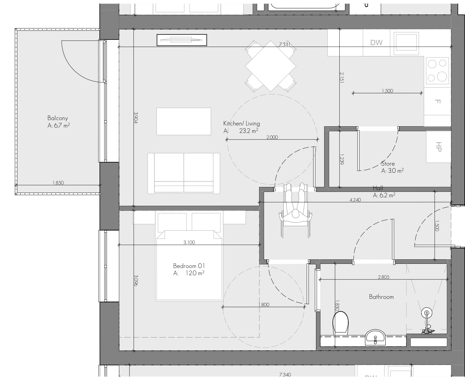
Apartment Type 1UD 1:50
