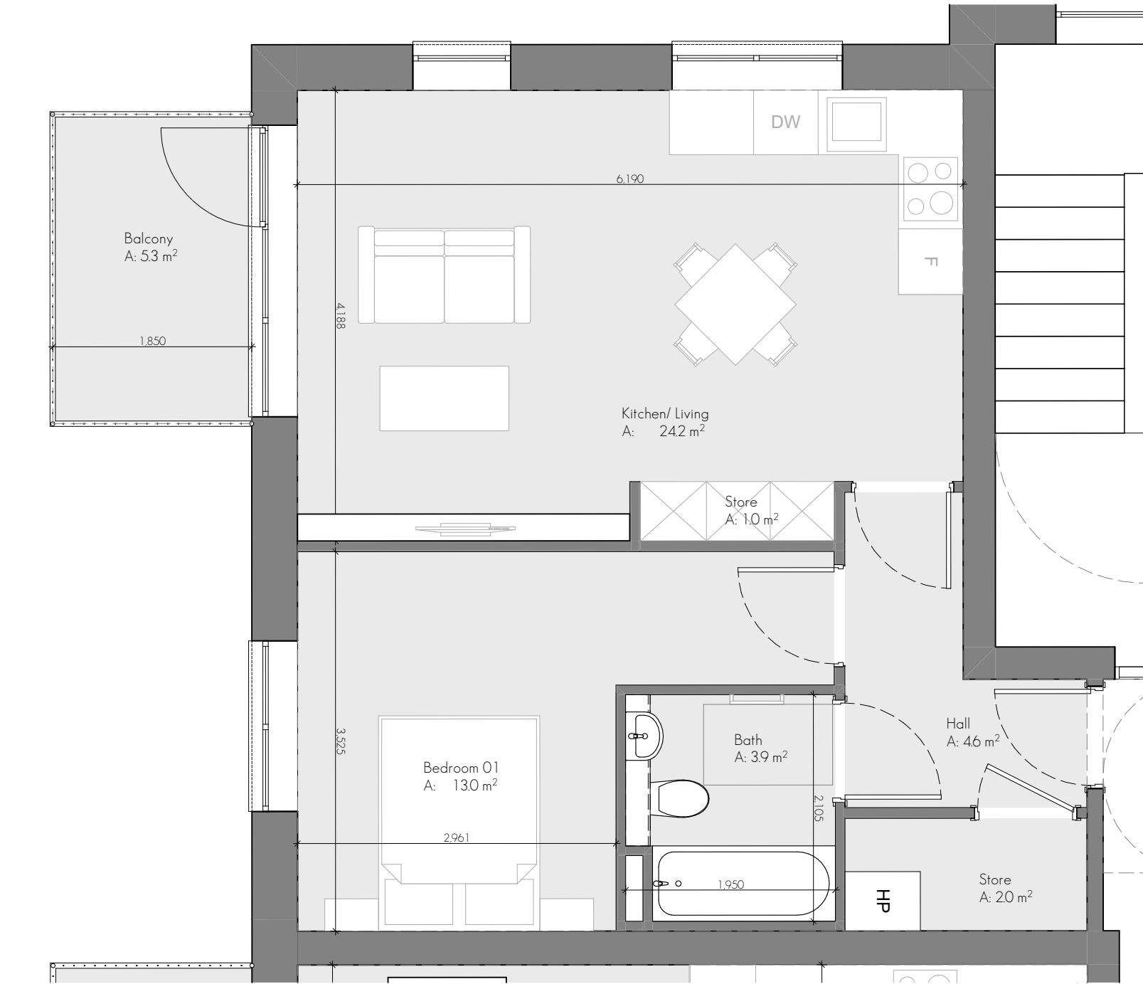
Apartment Type 1H 1:50
