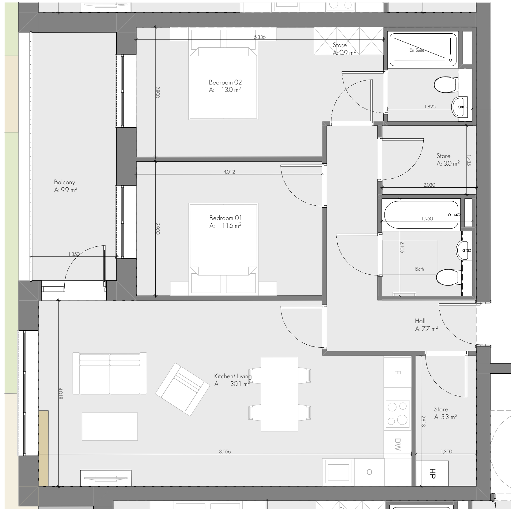
Apartment Type 2L 1:50
