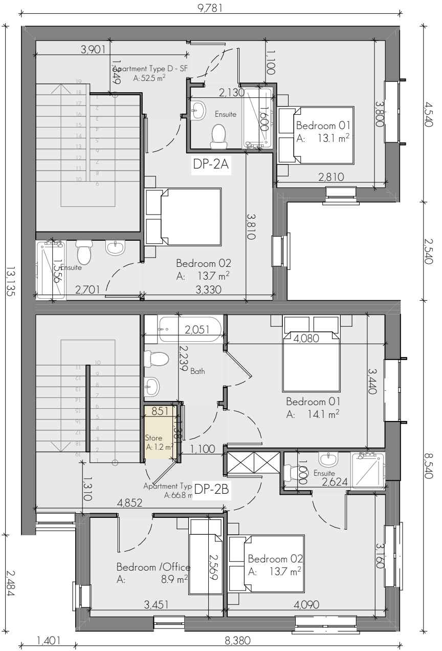
Second Floor 1:100
