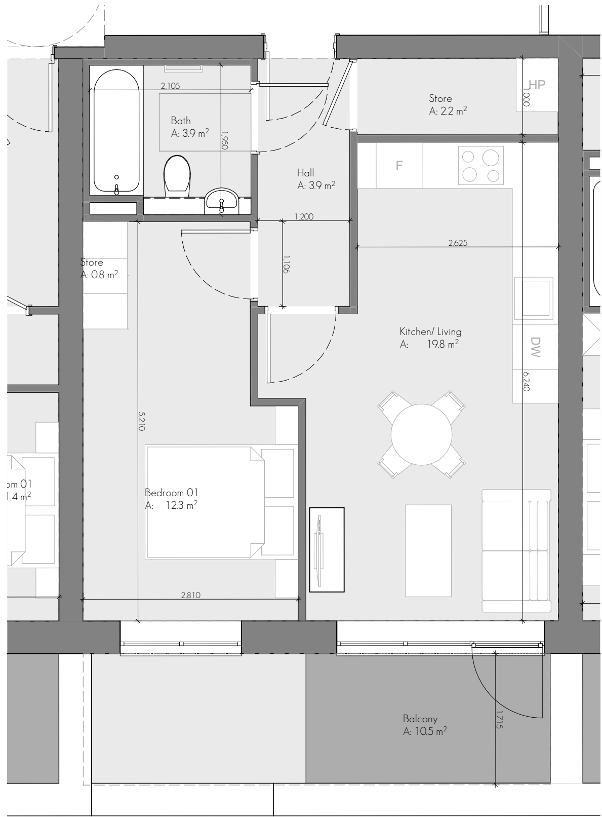
Apartment Type 1G 1:50
