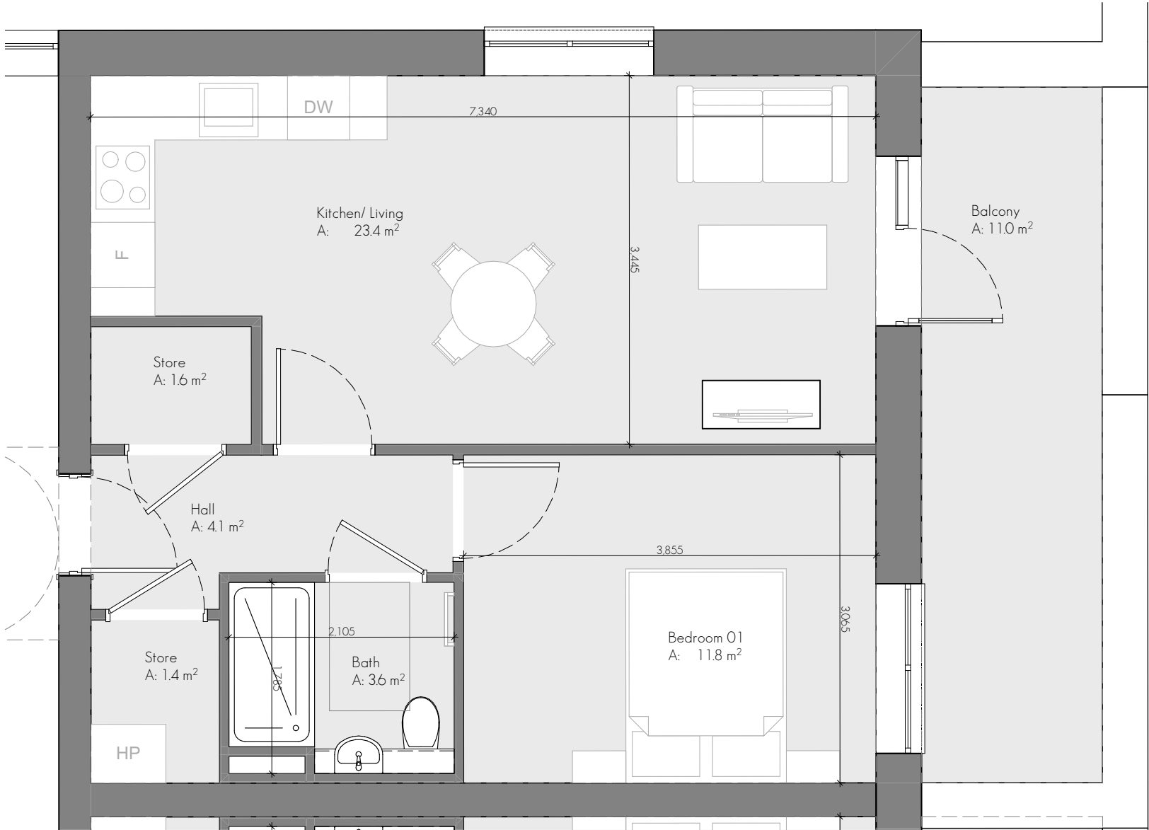
Apartment Type 1I 1:50
