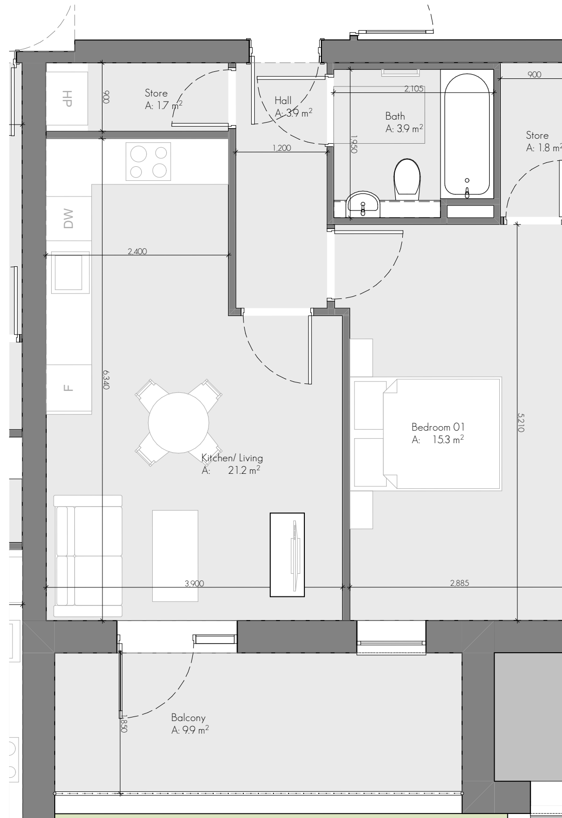
Apartment Type 1F 1:50
